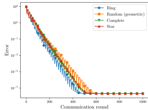
Fig. 2. Performance of LT-ADMM applied to different network topologies.
