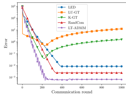
Fig. 3. Comparison over a network with quantized communications.
