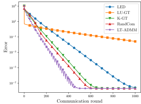
Fig. 1. Comparison of distributed optimization algorithms with local training.
