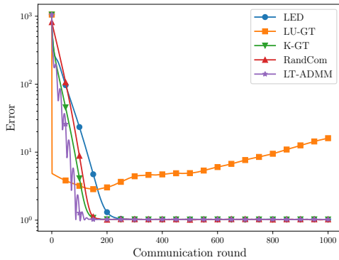
Fig. 4. Comparison using stochastic gradients with a batch of B = m_i/5 data points.
